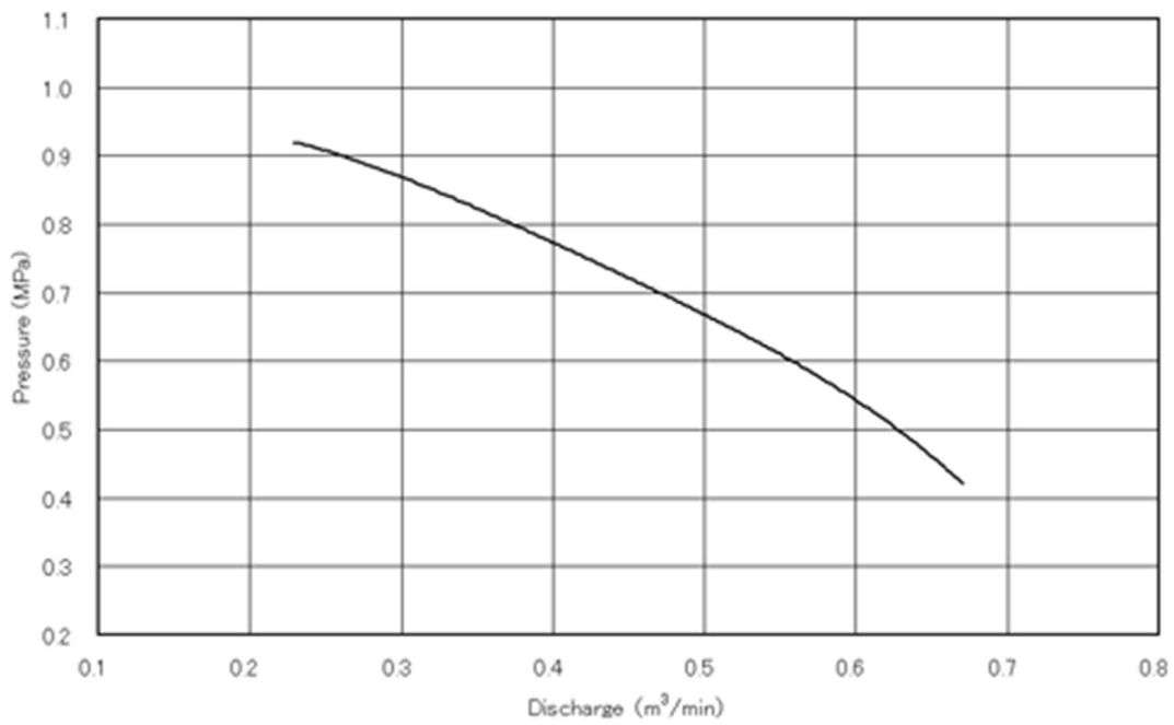
TF520 / Performance Curve
