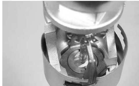
Correct Engagement for Model V36 Concealed/Recessed Wrench
