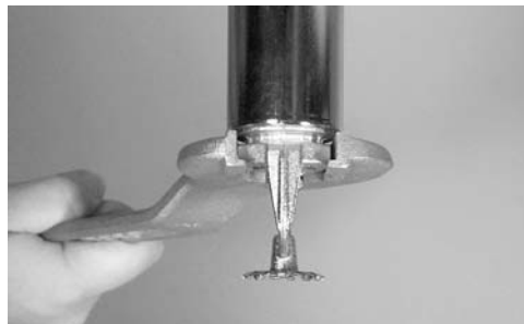
Correct Engagement for Model V36 Open-End Wrench
