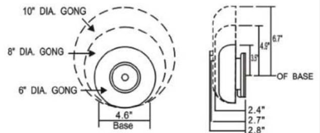
HC-1220 220 VAC
