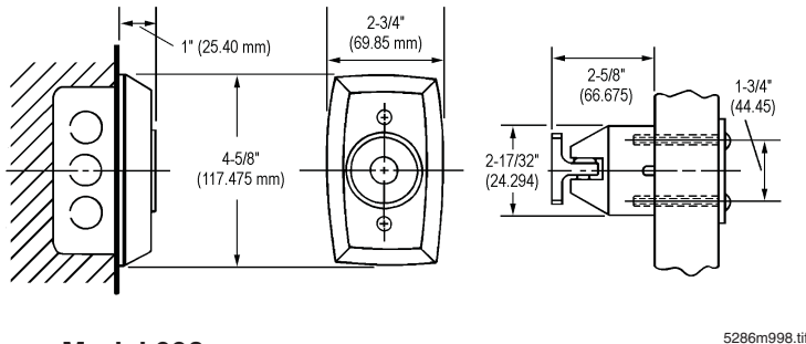
Model 998 Wall-Mount Standard Doors Concealed Wiring
