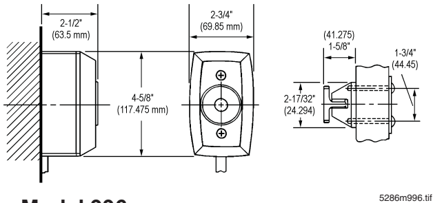
Model 996 Wall Mount Surface Wiring
