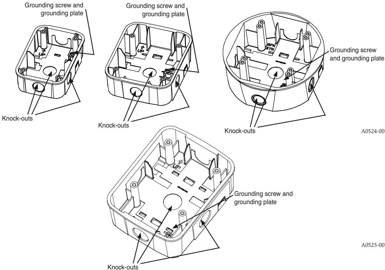
FIGURE 1. SURFACE MOUNT BACK BOX
