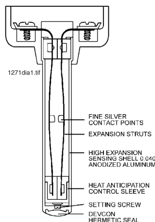
Cut-Away View
