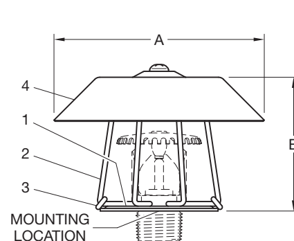
MODEL G6/S3 GUARD WITH SHIELD WITH EXAMPLE 3/4" NPT UPRIGHT MODEL K11-231B SPRINKLER
