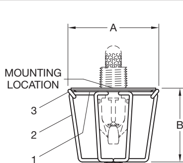
MODEL G1 GUARD WITH EXAMPLE 1/2" NPT PENDENT STAINLESS STEEL TYPE AM6 NOZZLE
