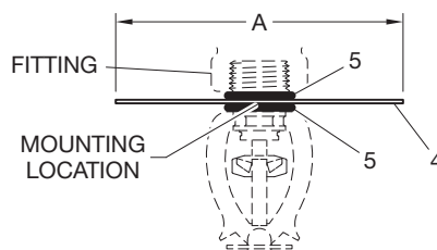
MODEL S4 SHIELD WITH EXAMPLE 1/2" NPT PENDENT SERIES TY-FRL SPRINKLER
