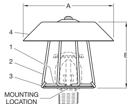
MODEL G4/S3 GUARD WITH SHIELD WITH EXAMPLE 3/4" NPT UPRIGHT SERIES TY-L SPRINKLER
