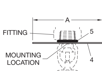
MODEL S2 SHIELD WITH EXAMPLE 1/2" NPT PENDENT SERIES TY-B SPRINKLER
