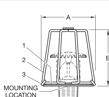
MODEL G6 GUARD WITH EXAMPLE 3/4" NPT UPRIGHT MODEL K11-231FRB SPRINKLER
