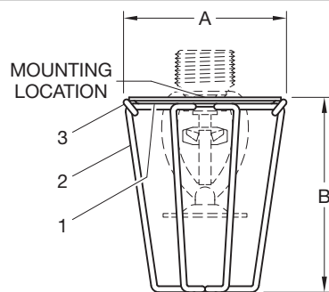
MODEL G4 GUARD WITH EXAMPLE 3/4" NPT PENDENT SERIES TY-FRL SPRINKLER
