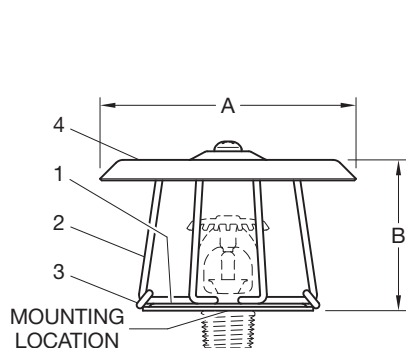
MODEL G1/S1 GUARD WITH SHIELD WITH EXAMPLE 1/2" NPT UPRIGHT SERIES TY-B SPRINKLER
