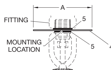
MODEL S5 SHIELD WITH EXAMPLE 1/2" NPT PENDENT SERIES TY-L SPRINKLER
