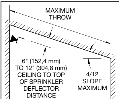
FIGURE 4 SPRINKLER PLACEMENT UNDER SLOPED CEILINGS IN LOADING DOCKS
